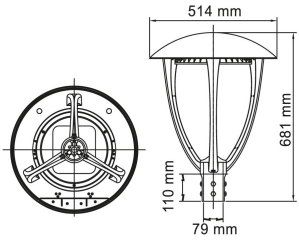
Faroled 80W
