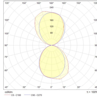
Roadlight 3W 180°
