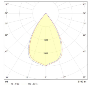
Downlight 34W 60°
